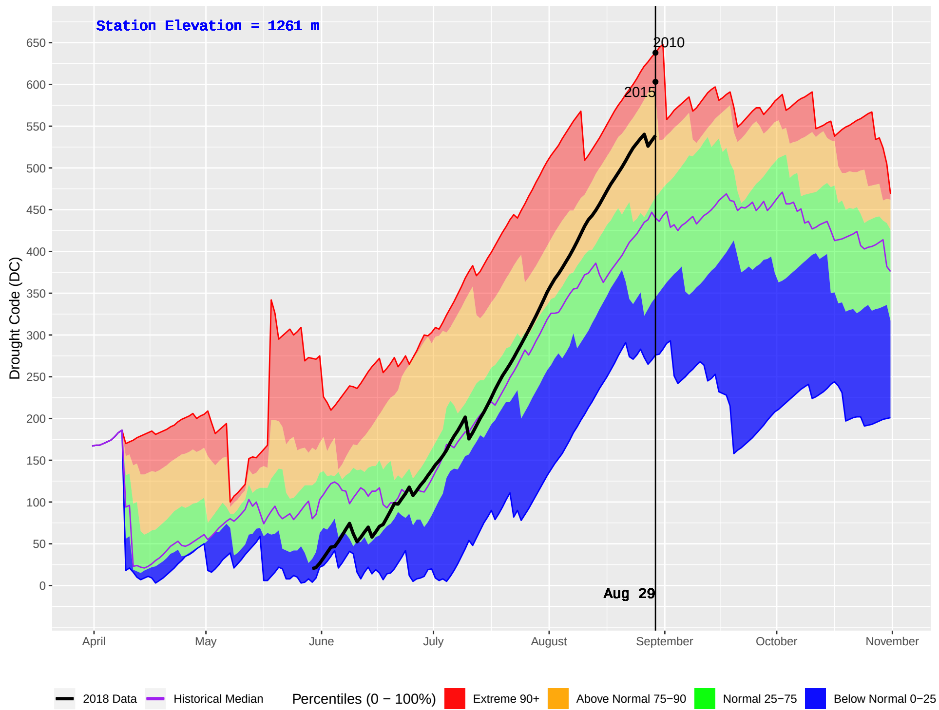
IDA BELL LAKE 3 (876) : Historical (2004–2016) and Current (2018) Daily Drought Code (DC)
