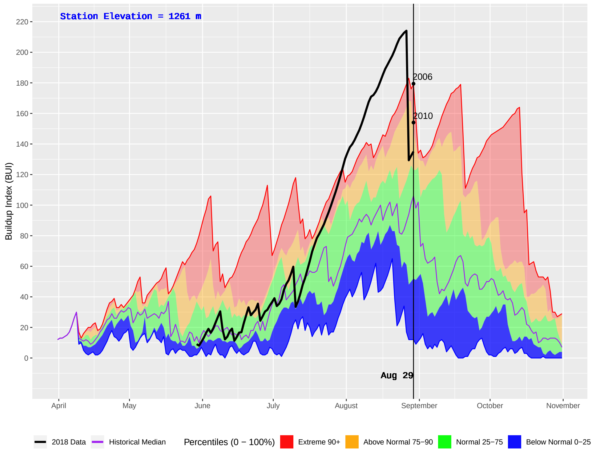
IDA BELL LAKE 3 (876) : Historical (2004–2016) and Current (2018) Daily Buildup Index (BUI)
